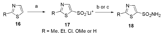
Scheme 4. Reagents and conditions: (a) (i) n -BuLi, THF, -78^{\circ}\text{C} ; (ii) \text{SO}_2 , -78^{\circ}\text{C} to rt; (b) for R = Me, Et, or Cl: (i) NCS; (ii) \text{NH}_4\text{OH} ; (c) for R = OMe or H: \text{H}_2\text{NOSO}_3\text{H} , NaOAc.
